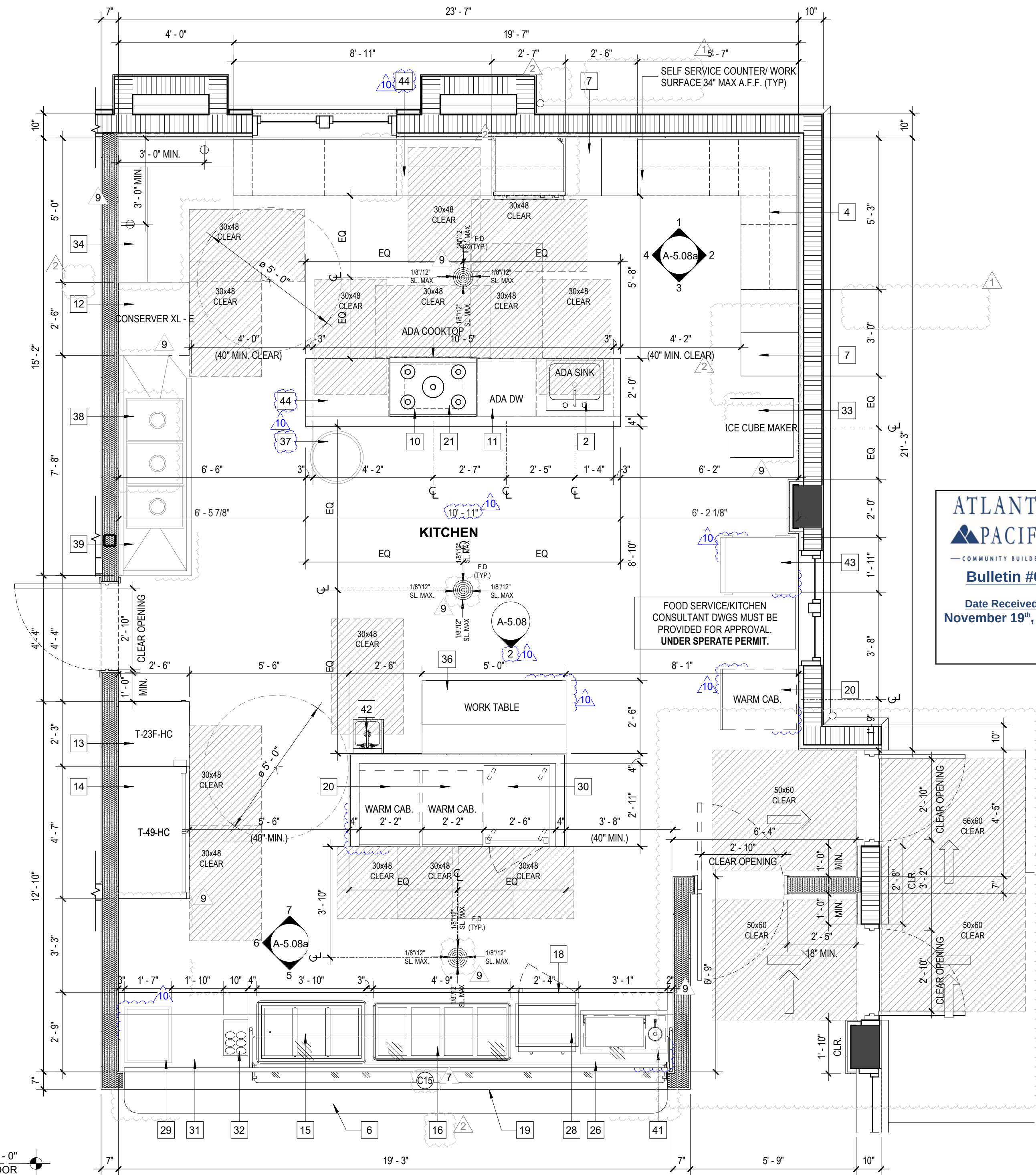
1 COMMUNITY CENTER KITCHEN SCALE: 3/8" = 1'-0"
