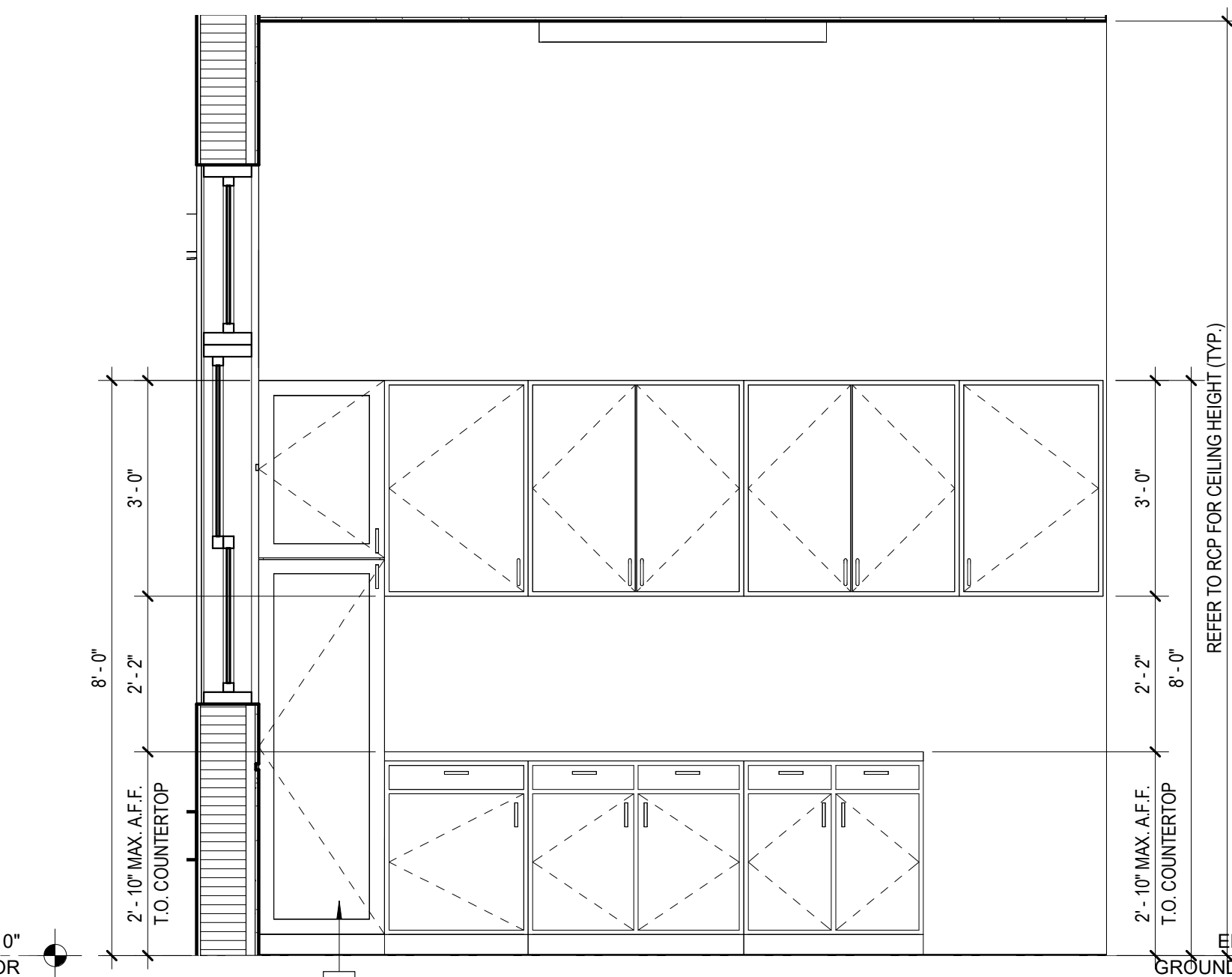
7 COPY/FILE ROOM ELEVATIONS SCALE: 1/2" = 1'-0"
