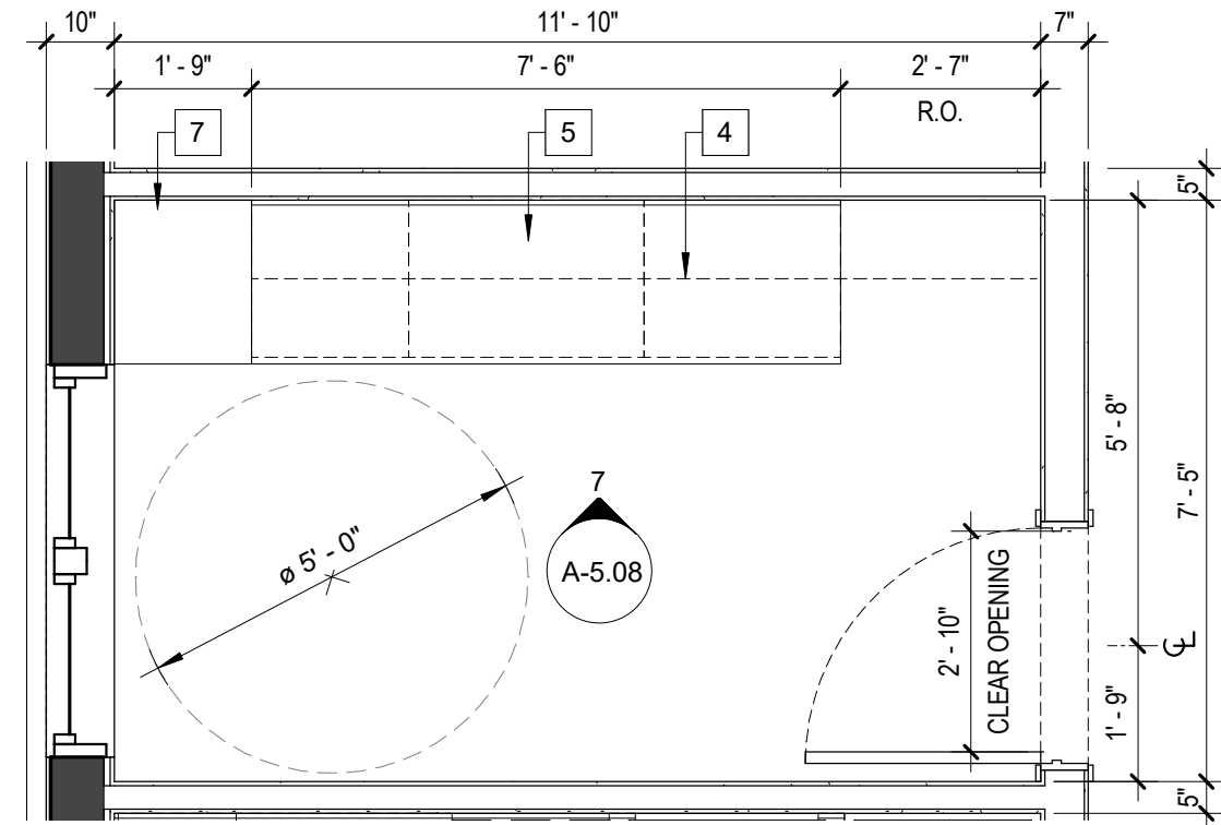
4 COMMUNITY CENTER COPY/FILE ROOM SCALE: 3/8" = 1'-0"
