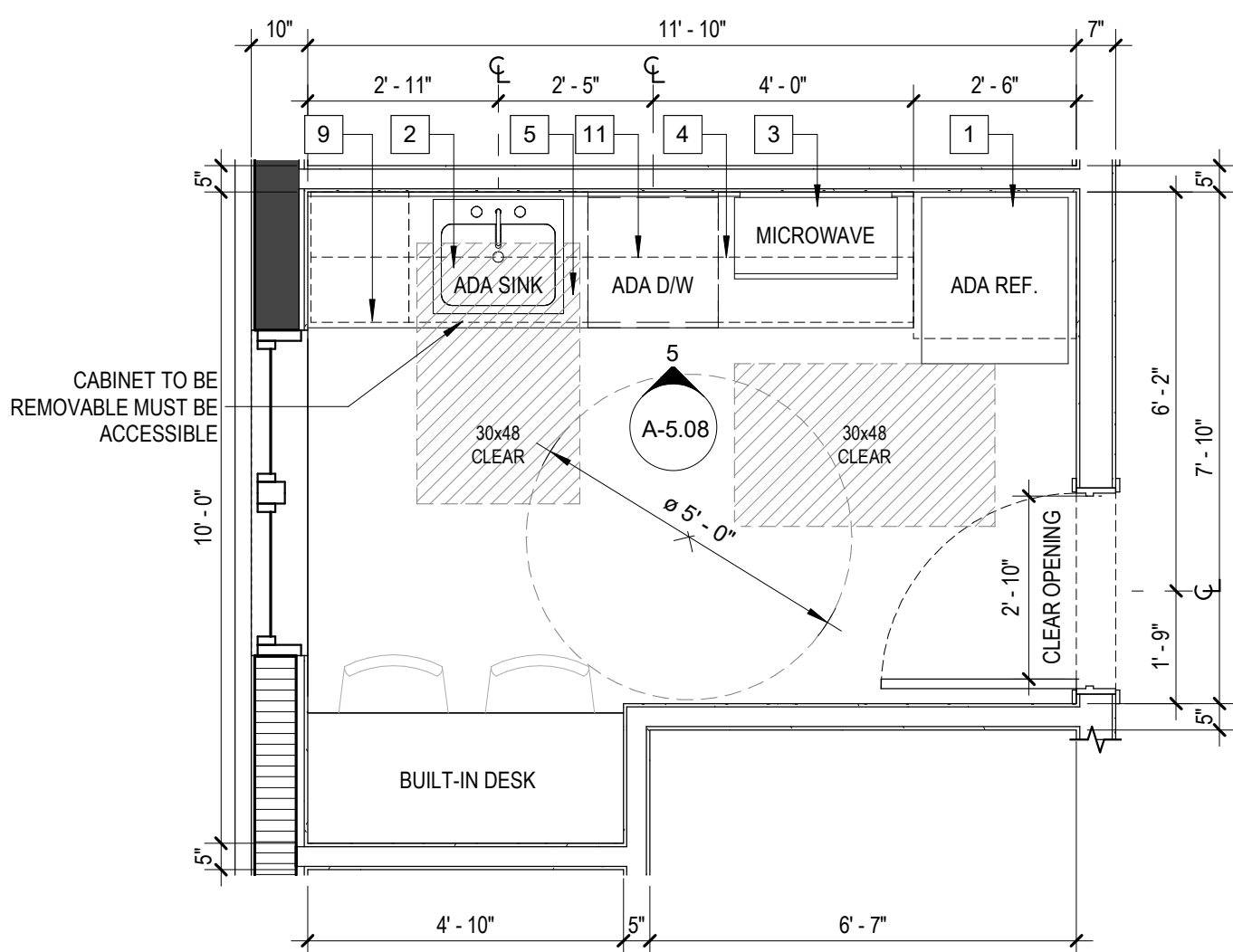
3 COMMUNITY CENTER BREAK ROOM SCALE: 3/8" = 1'-0"
