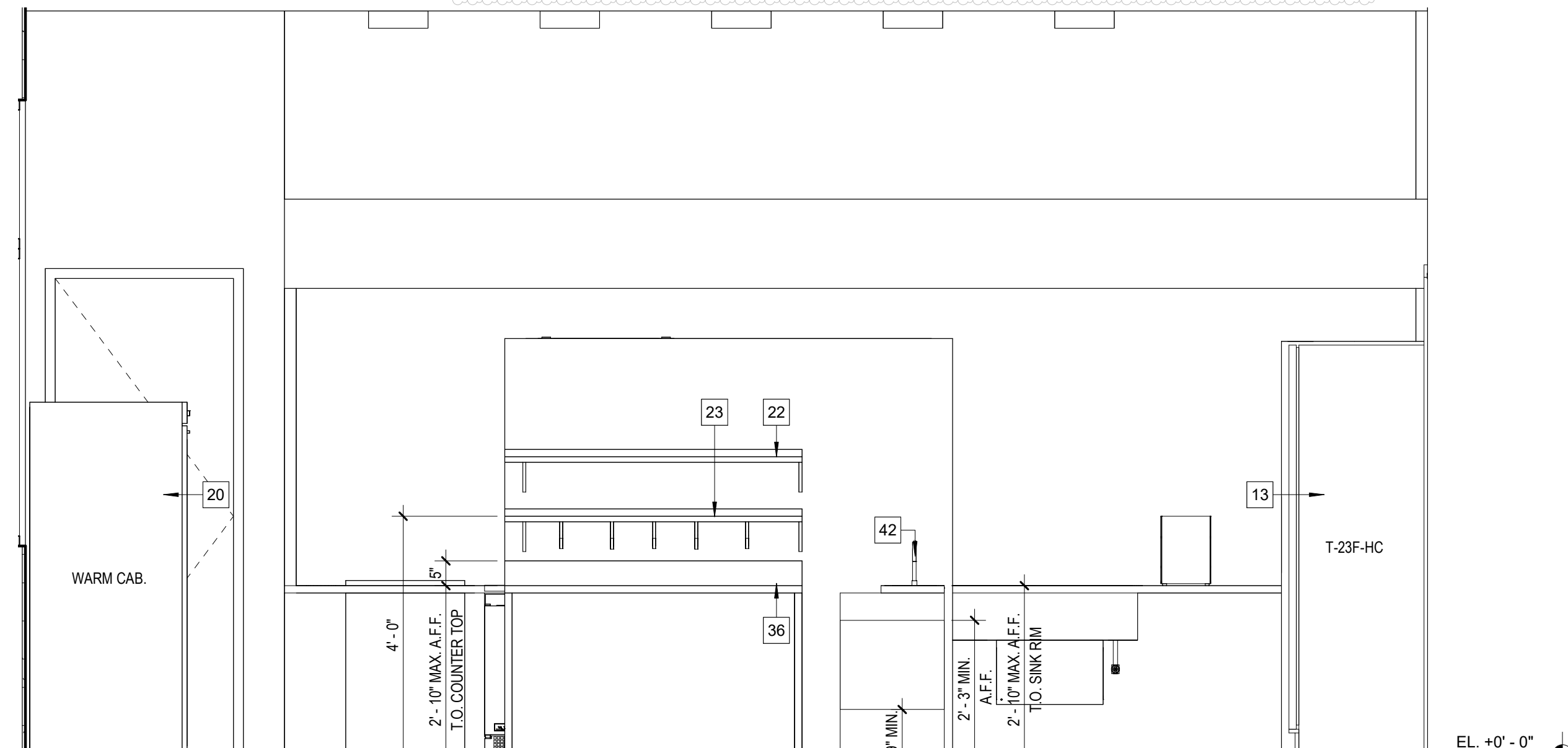
1 COMMUNITY CENTER KITCHEN SCALE: 3/8" = 1'-0"
