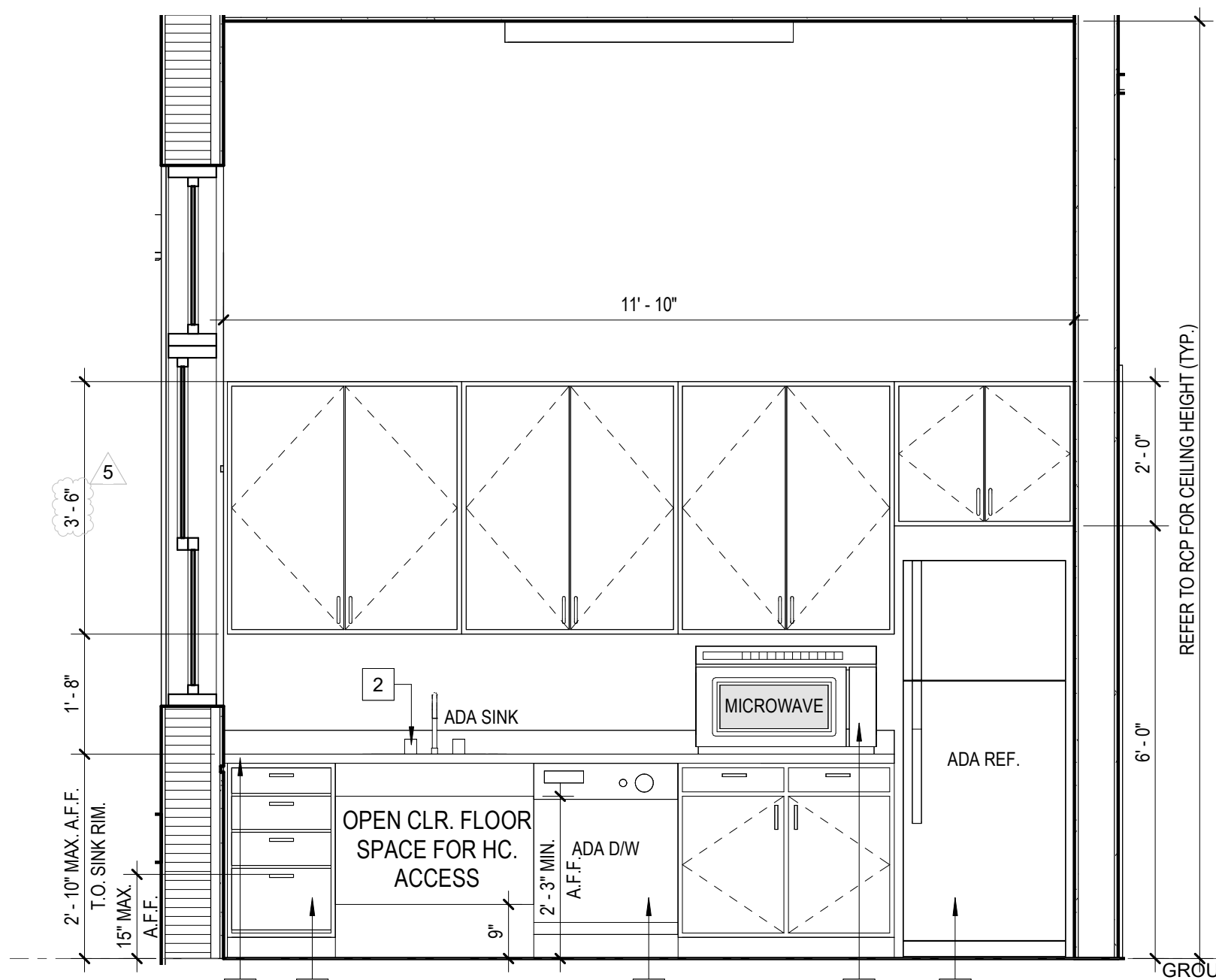
5 BREAK ROOM NORTH ELEVATION SCALE: 1/2" = 1'-0"
